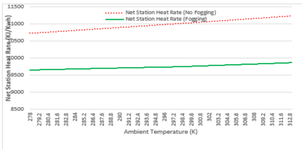
Figure8. Effect of ambient temperature on heat rate
