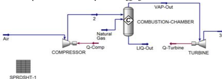
Figure1. Flow chart of simulated simple gas turbine
