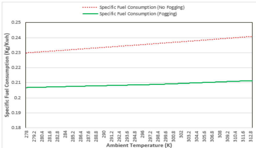
Figure7. Effect of ambient temperature on specific fuel consumption
