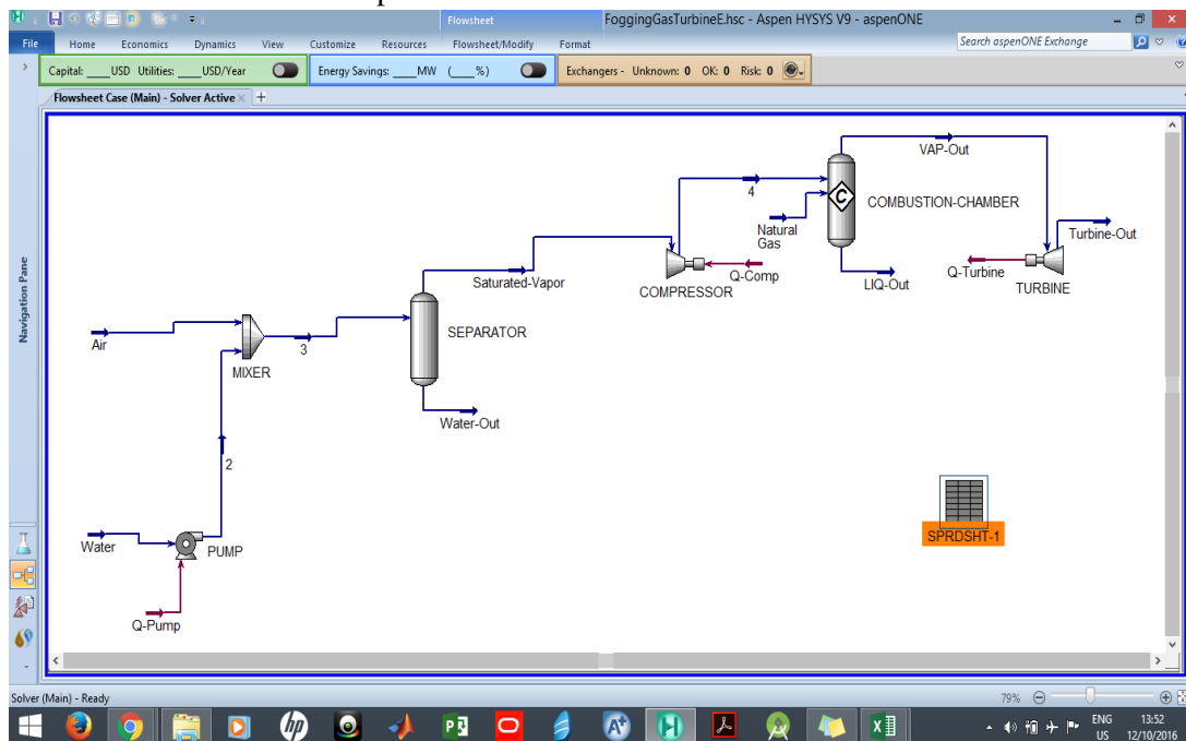
Figure3. Process Flow sheet for Gas Turbine with Fogging Unit.
