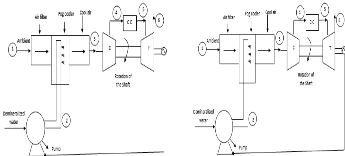
Figure2. Schematic diagram of fogging unit incorporates to gas turbine
