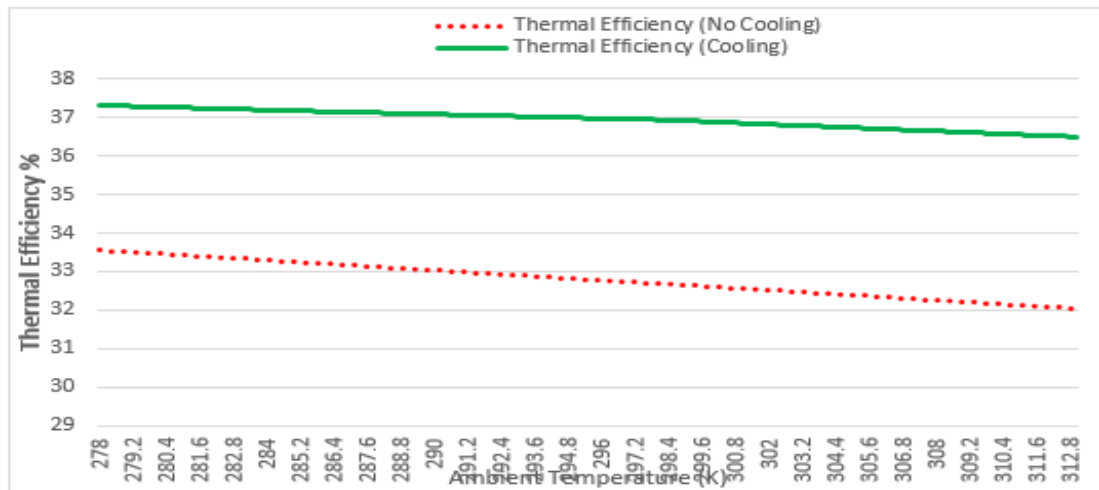
Figure 5. Effect of ambient temperature on thermal efficiency of gas turbine plant
