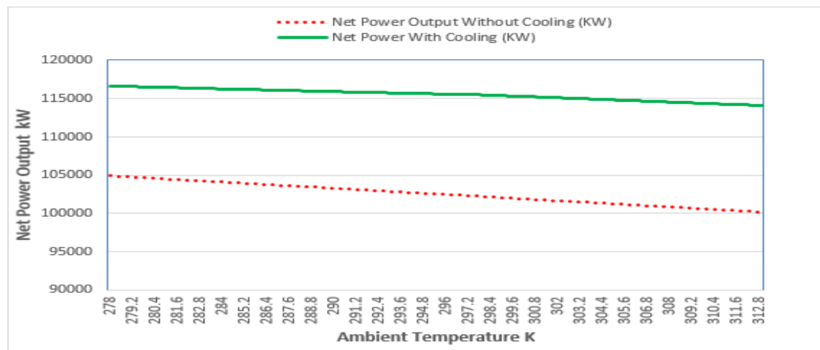
Figure 6. Effect of ambient temperature on net power output
