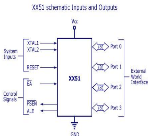
Figure1. Schematic diagram of 8051 microcontroller
