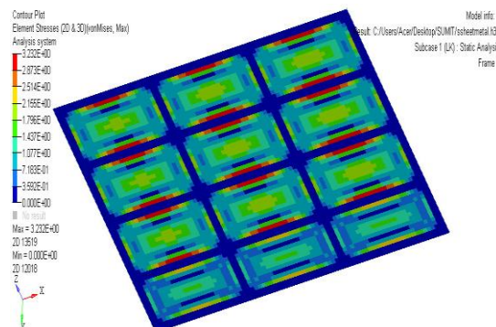
Figure2. Analysis for the bottom plate of the tank with the help of Hypermesh 11.0
